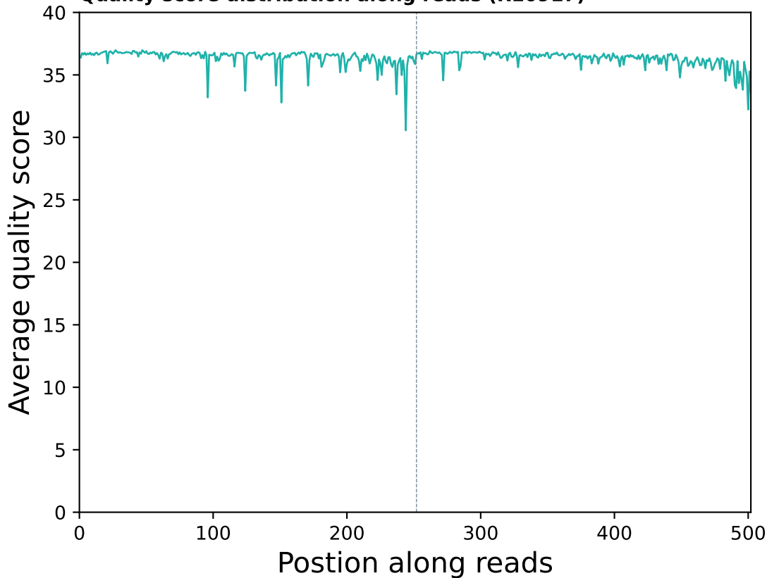
Quality score distribution along reads (R10917)
